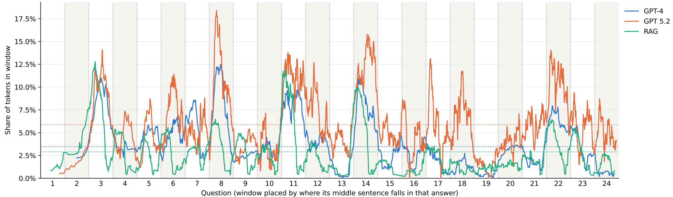
Negative: DocuScope 25-sentence moving window by model. Dotted: whole-text value.
