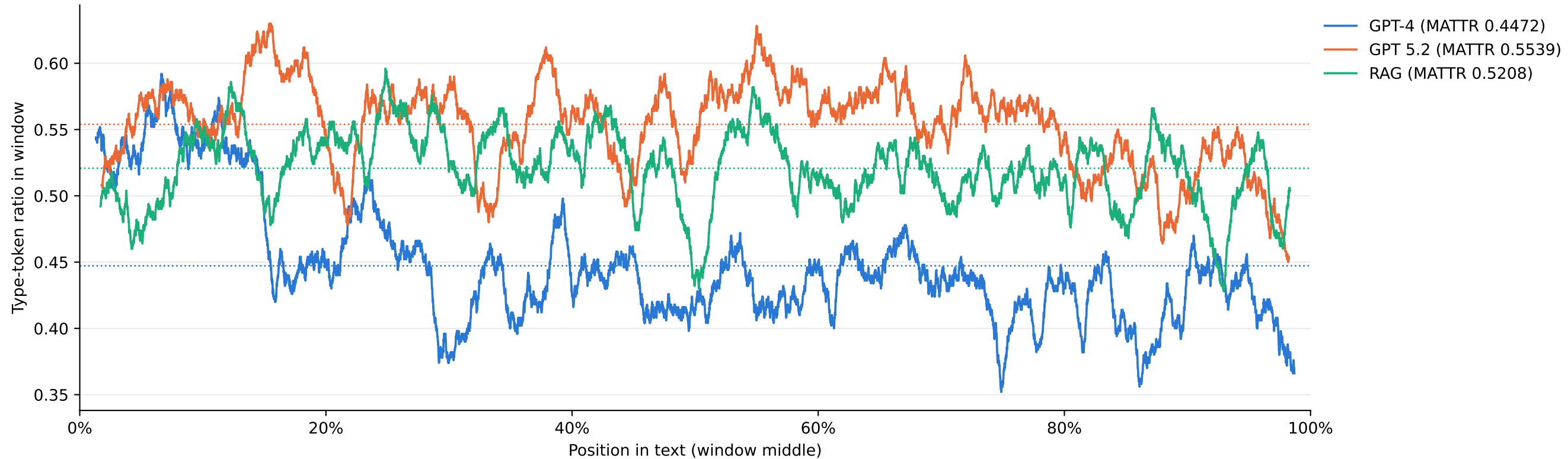
MATTR: 500-lemma moving window by model. Dotted: mean over all windows (the model's MATTR).
