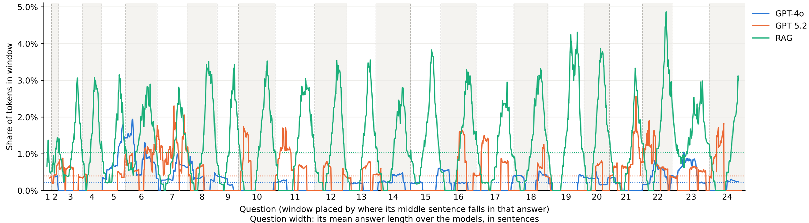
Citation: DocuScope 25-sentence moving window by model. Dotted: whole-text value. Each window is assigned the question its middle sentence comes from.
