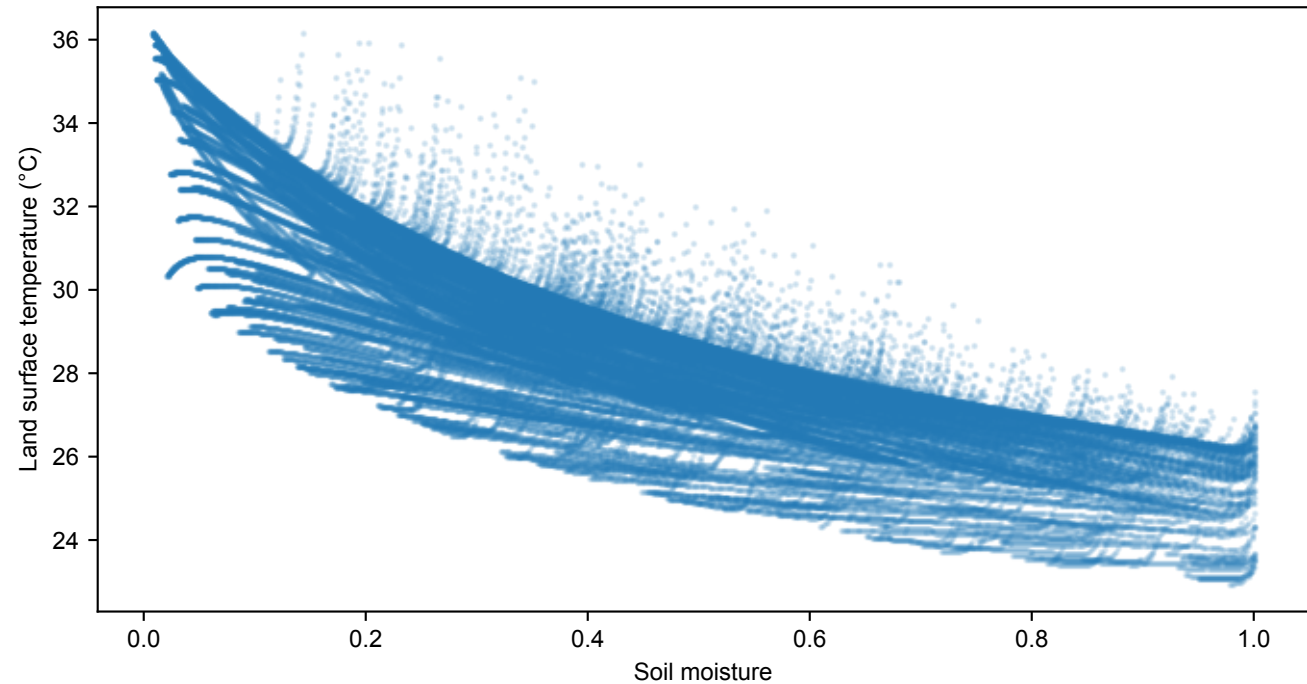
JJA soil moisture-temperature relationship
