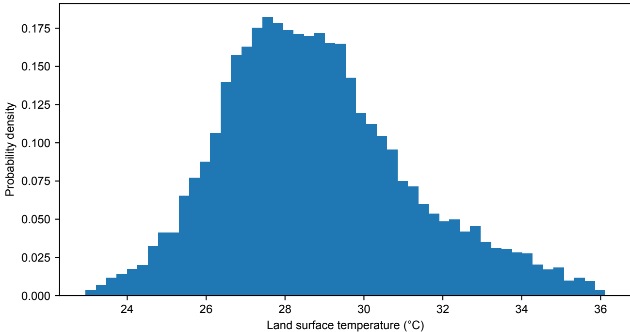
JJA land temperature
