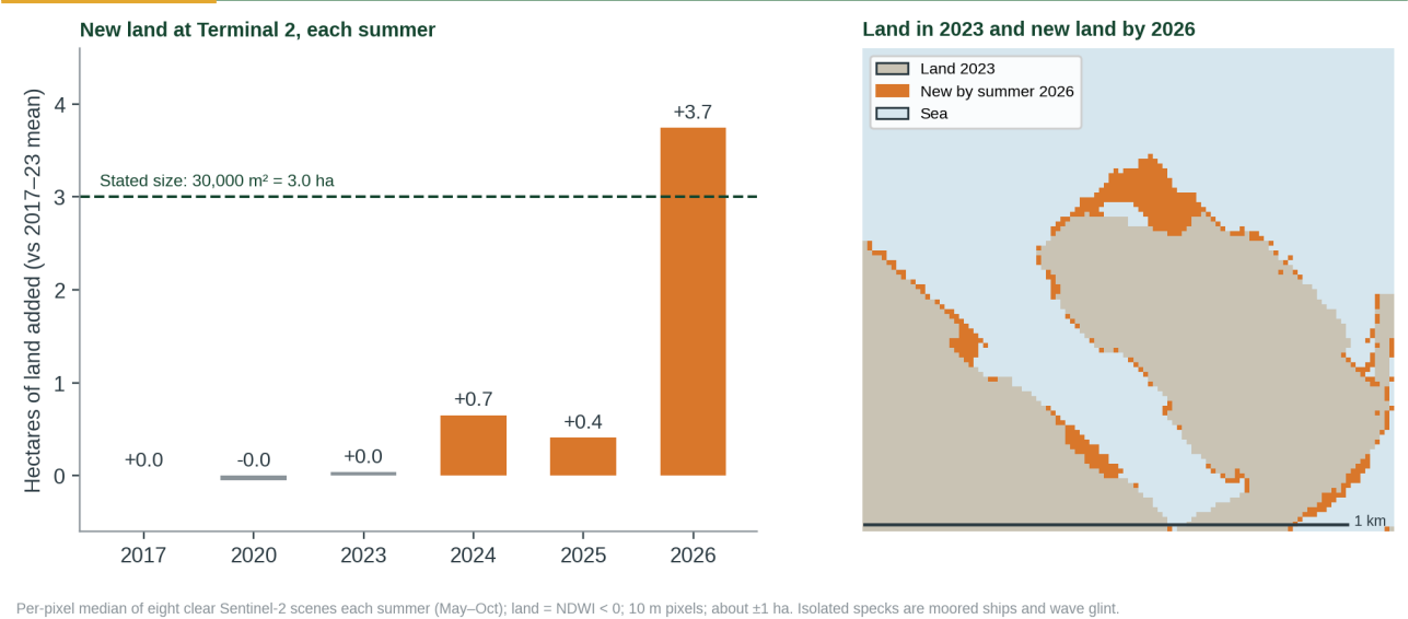
Figure 1. Land at Freeport Terminal 2 from Sentinel-2. No change 2017–2023; new land from 2024, about 3.7 ha by summer 2026, close to the stated 30,000 m² [5, 6].
