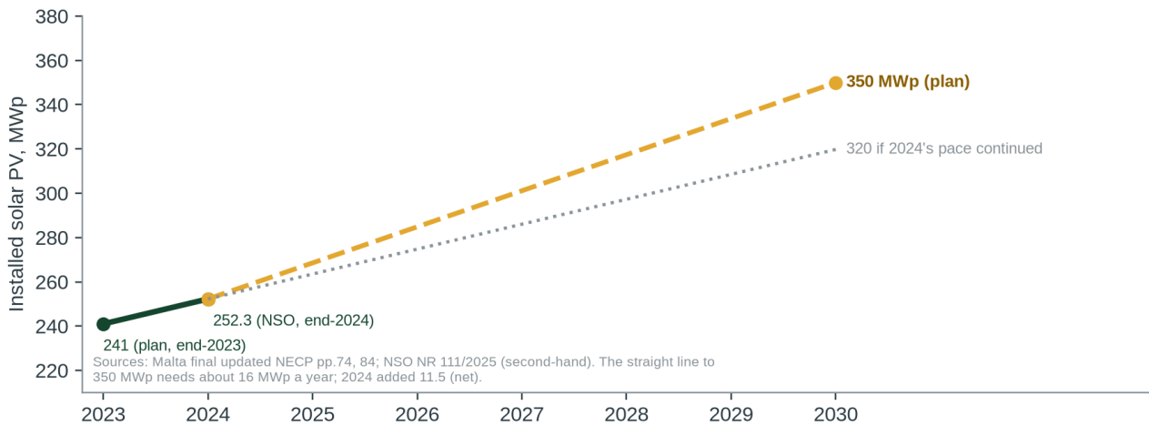
Figure 3. Installed solar PV: plan's 350 MWp path against the 2024 pace. NSO figures are second-hand.
