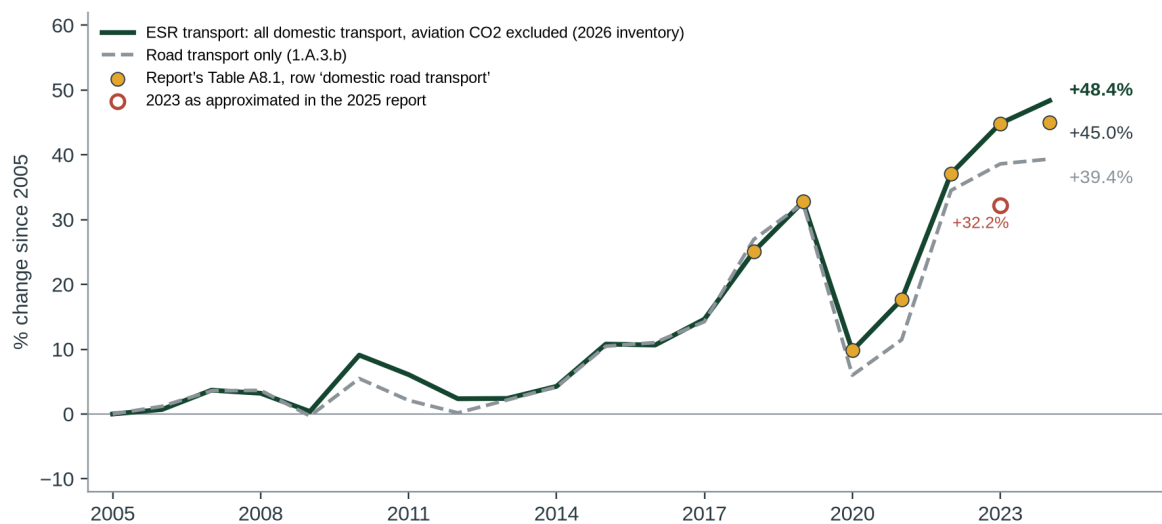
Greenhouse gases, CO 2 equivalent. Source: Eurostat env_air_gge (2026 inventory, updated 2 Jun 2026; no flags on these rows); Commission 2026 and 2025 Country Reports (Table A8.1). The 2024 Table A8.1 value rests on the approximated inventory (our recomputation from it: +44.1%). Retrieved or read 6 Oct 2026.
