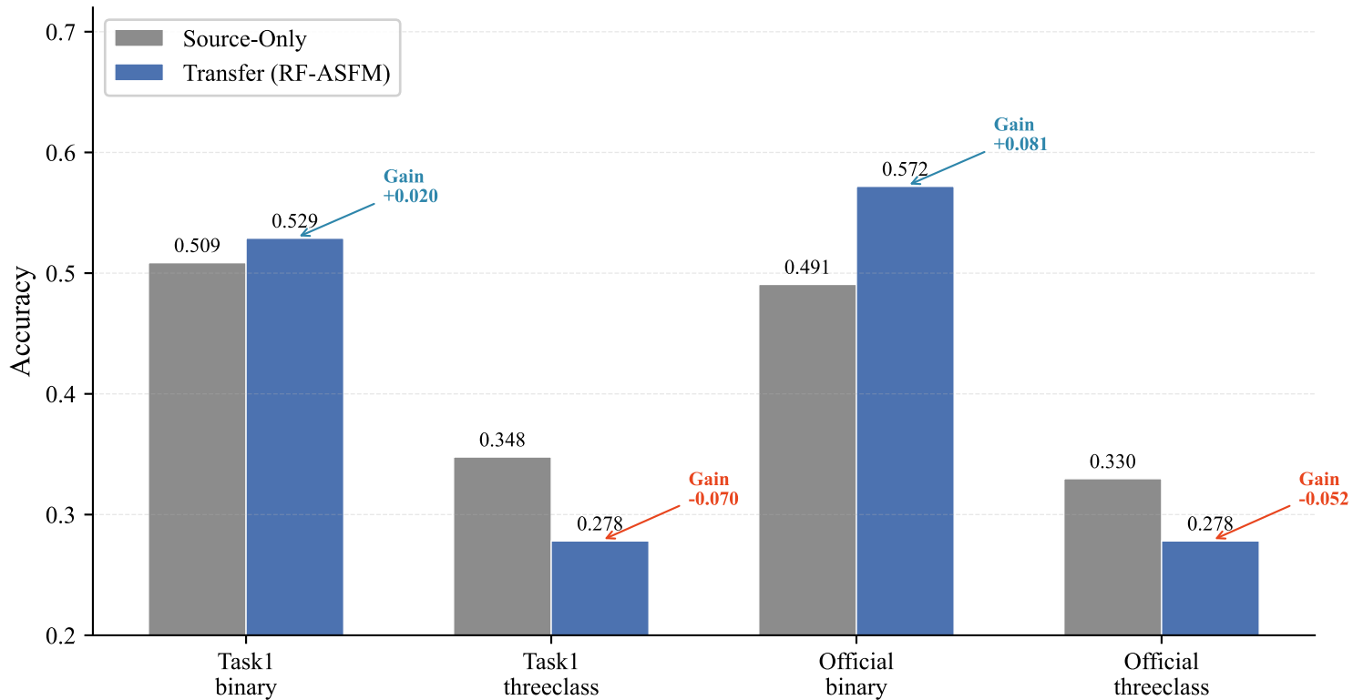
Source-Only vs Transfer Accuracy (RF-ASFM)
