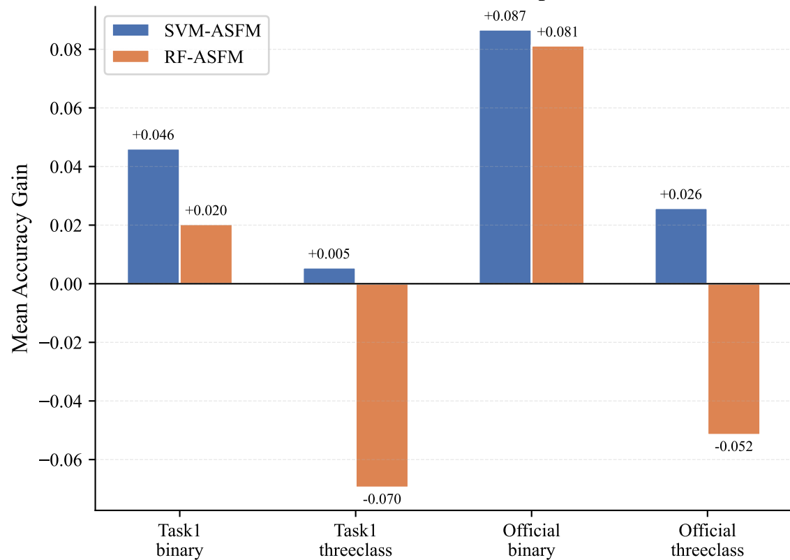
Mean Transfer Gain Comparison
