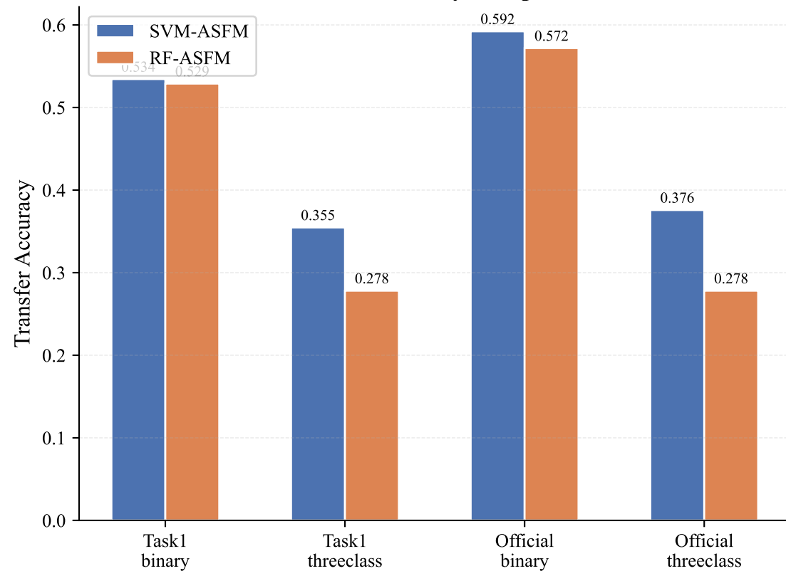
Transfer Accuracy Comparison
