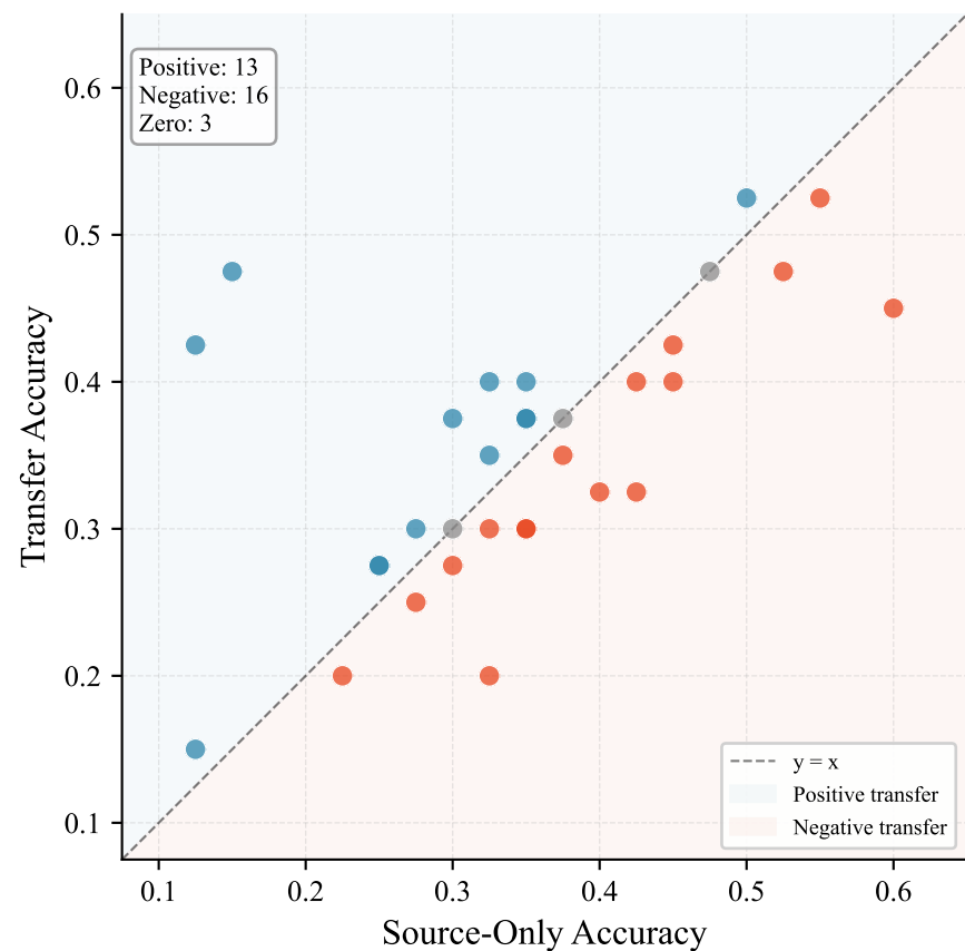
Official Threeclass
