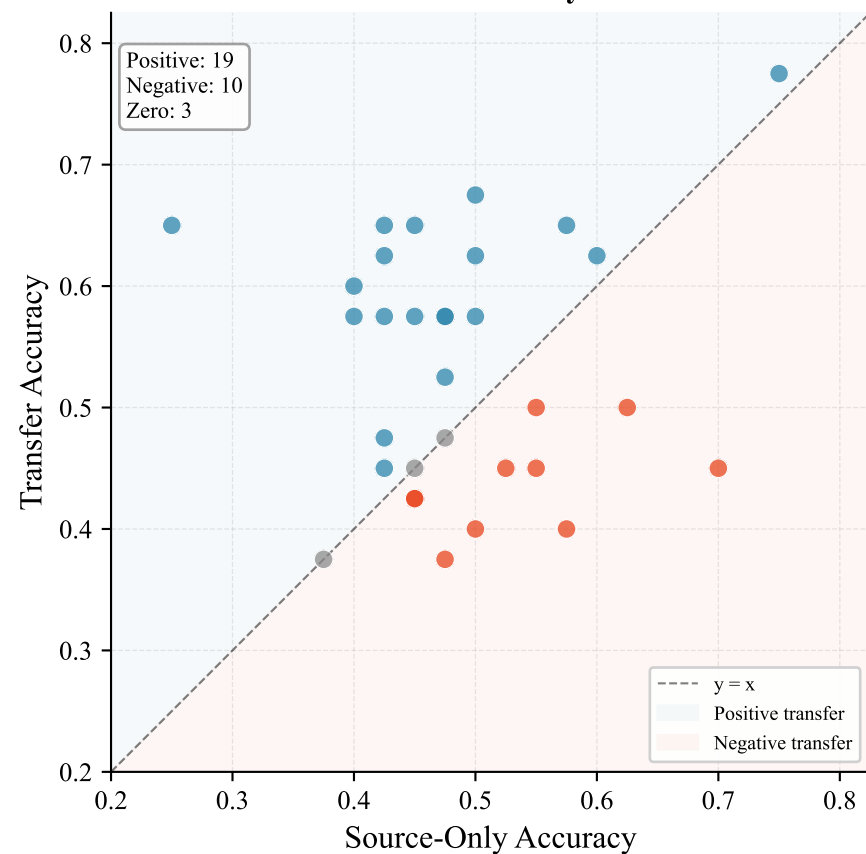
Official Binary
