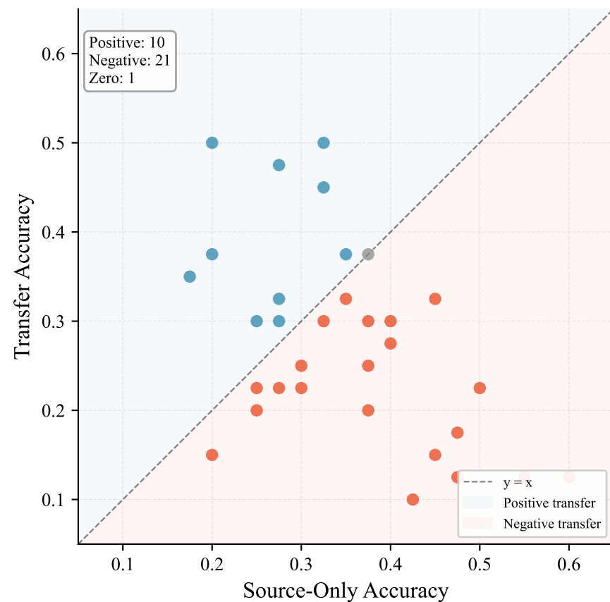
Official Threeclass
