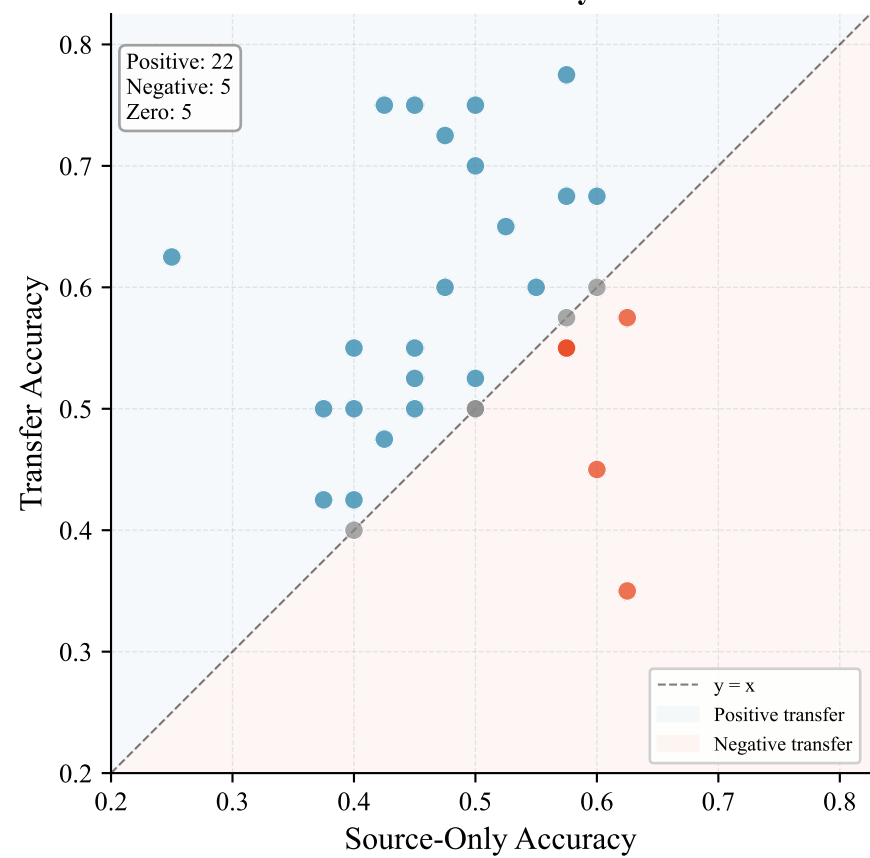
Official Binary
