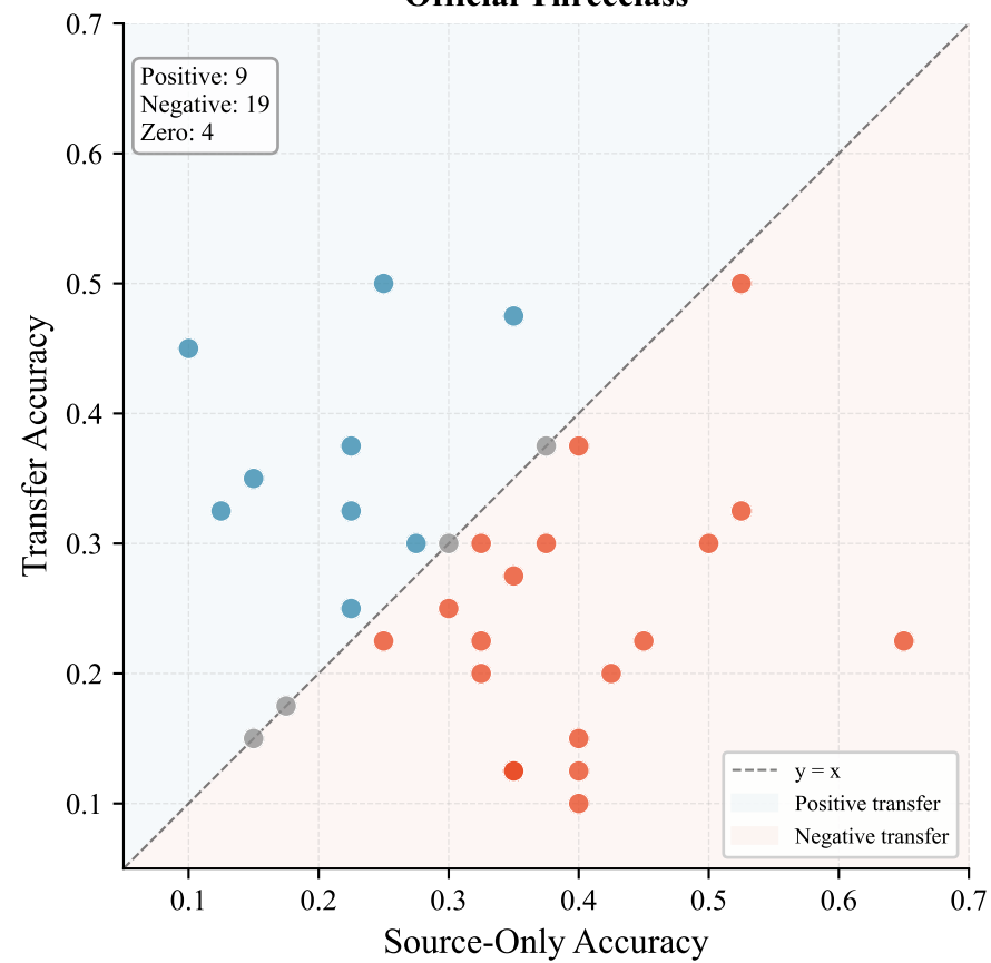
Official Threeclass
