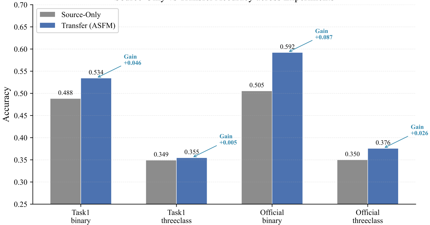
Source-Only vs Transfer Accuracy across Experiments
