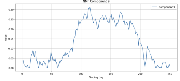
Figure 1: NMF component 9 of the yearly NASDAQ price matrix (normalised values, position of the trading day within the year).
