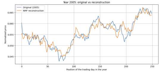
Figure 2: Original versus NMF-reconstructed normalised NASDAQ path for the year 2005 (in-sample).
