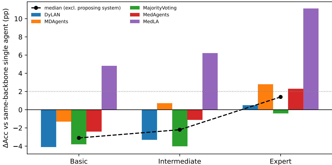
Multi-agent gain by item difficulty (MedDDx, LLaMA-3.1-8B)
