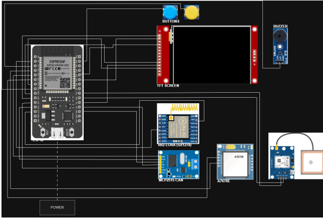
Figure 3: Embedded HMI hardware block showing the separation of OBD-II/CAN, GPS, display, radio, modem, and driver-control functions.
