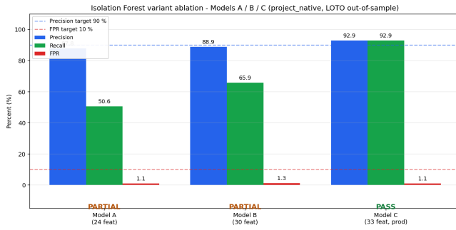
Figure 7: Model-performance comparison used to support the SO4 production-detector selection.
