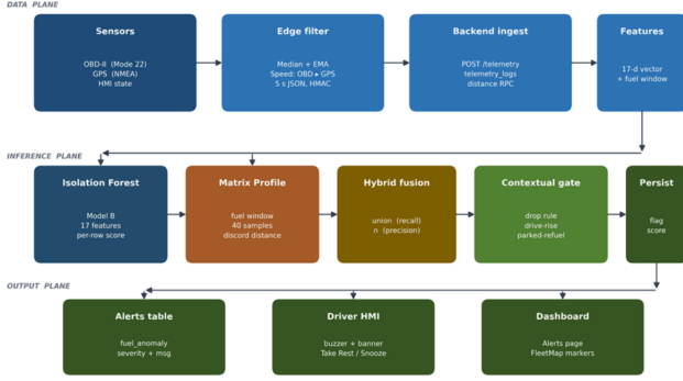
Figure 5: Machine-learning anomaly-detection architecture from filtered telemetry to model score, contextual gate, stored alert, and dashboard/HMI feedback.
