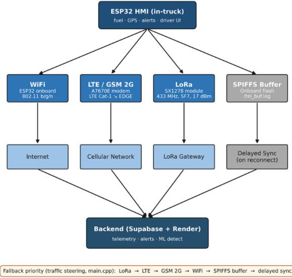
Figure 2: End-to-end edge-to-cloud system architecture.
