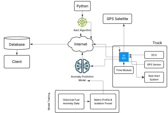
Figure 1: Conceptual diagram of the IoT-enabled fuel monitoring and anomaly-detection system.
