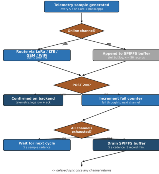
Figure 6: Offline-buffer fall-through path used when live communication channels are unavailable.
