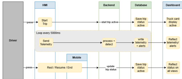
Figure 8: Cross-interface trip-state synchronization between HMI, backend, database, dashboard, and mobile surface.
