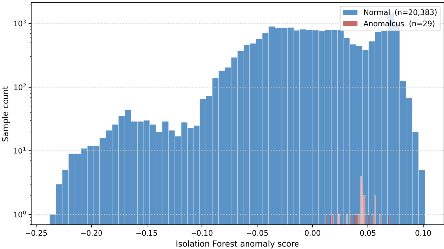
Fig. 6.20 Anomaly Score Distribution
