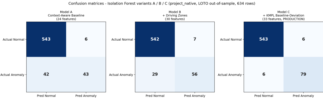
Fig. 6.21 Confusion Matrices: Models A, B, and C
