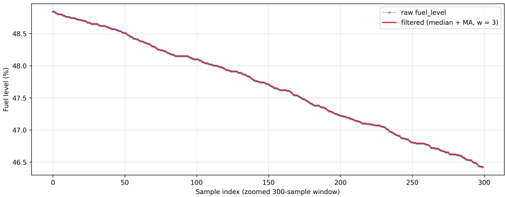
Fig. 6.9 Filtering Effect: Raw versus Filtered (Zoomed)
