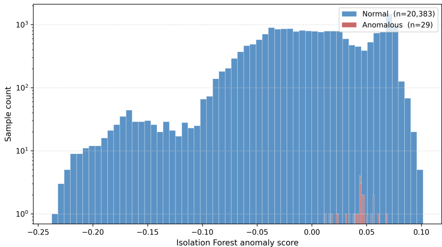
Fig. 6.19 Anomaly Score Distribution
