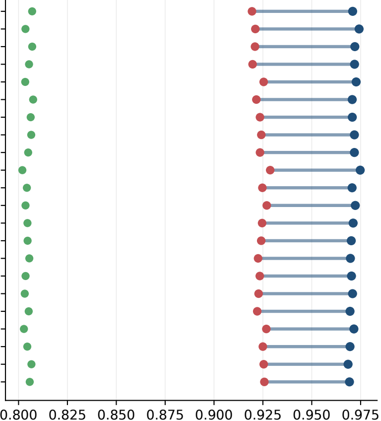
(e) 15% masked
