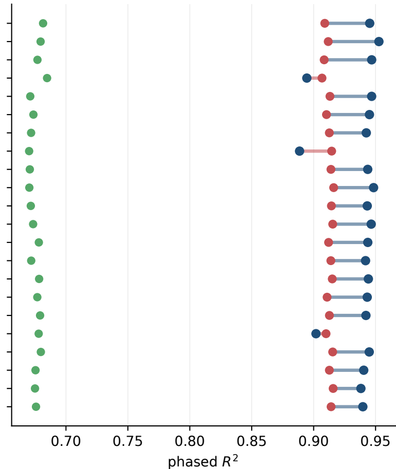
(f) 25% masked
