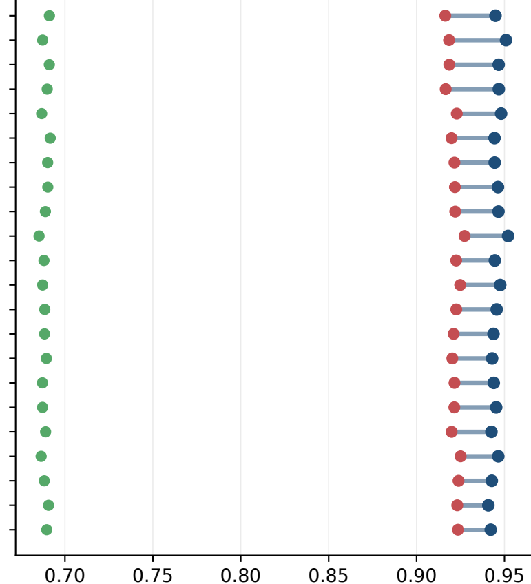
(f) 25% masked
