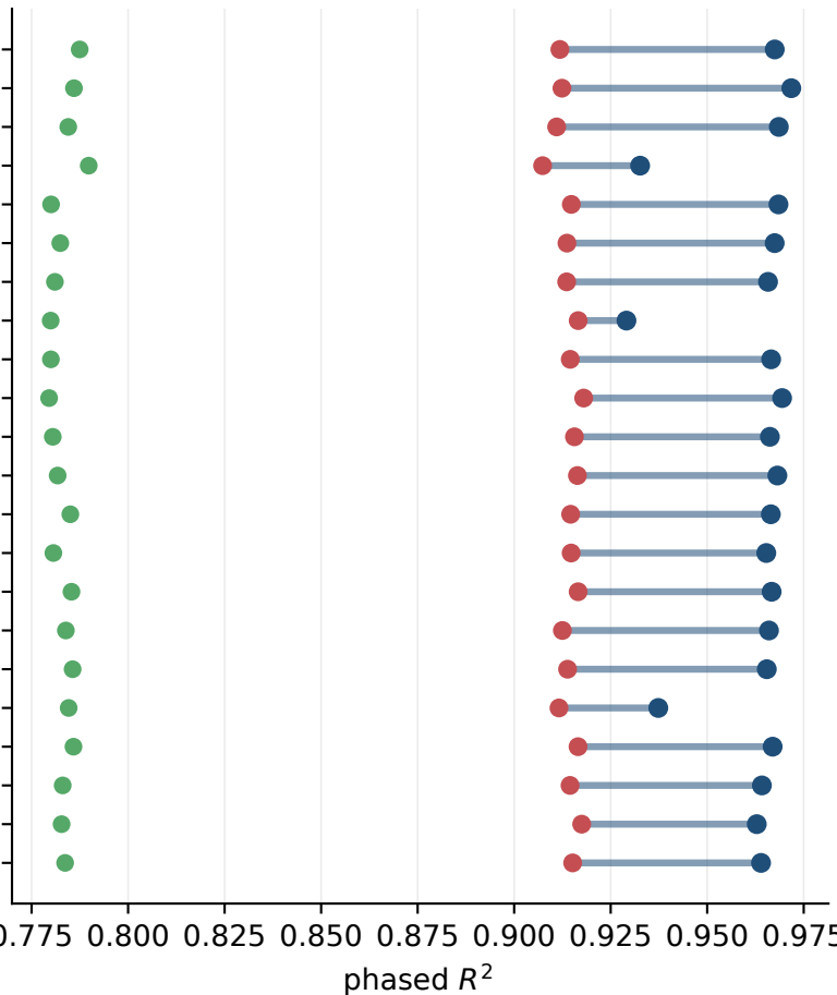
(e) 15% masked
