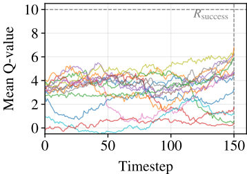
Truncated (n=15)
