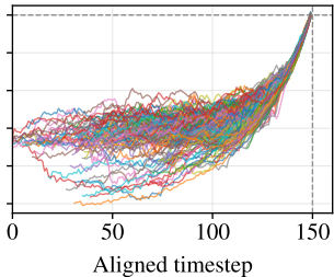
Successful (n=285)
