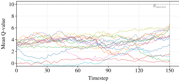
Truncated rollouts (n=15)
