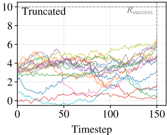
Mean Q-value
