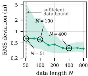
DeePC tracking error
