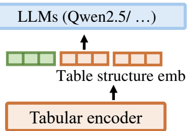
(b) (Hyper)Graph-based method
