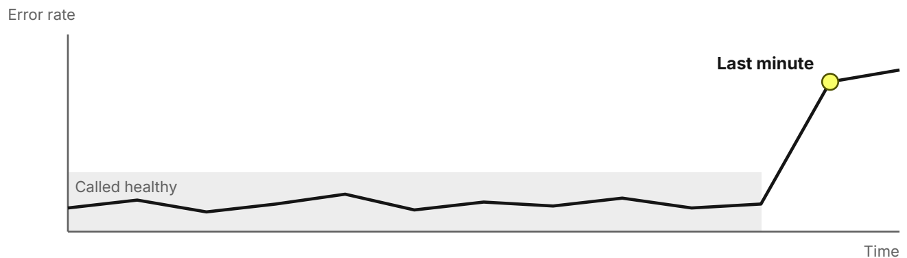
Figure 16 Every verdict is relative to the shaded stretch. Change it and every verdict changes.
