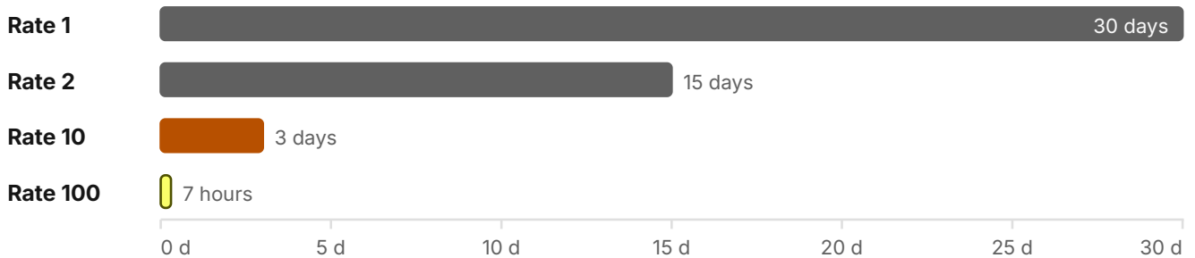
Figure 14 How long the whole budget lasts at each rate. Rate 1 is on target. Rate 100 is an outage.
