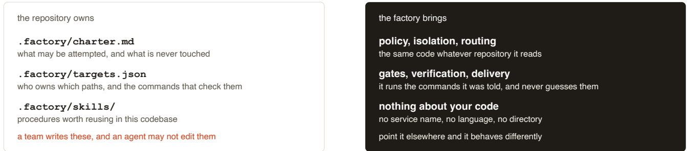
Figure 6. The split that makes a factory portable. Facts on the left, logic on the right, and the line between them is what a second repository tests.
