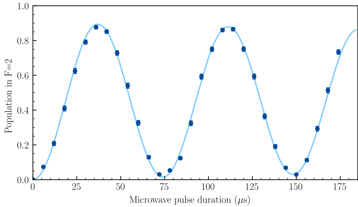
Figure 3.6: Rabi oscillations for the F = 1, m_F = 0 \leftrightarrow F = 2, m_F = 0 transition. The solid line represents the fit given by (3.1) to the data points.
