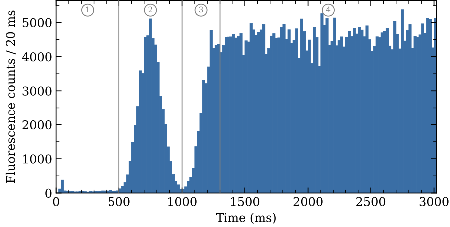
Figure 3.3: Typical trace in which fluorescence counts are recorded during the atom positioning procedure as a function of time. The MOT release sets the time = 0s. Around time 0.1s, an atom is trapped in the 852 nm trap and is not coupled to the cavity (1). Around time 0.5 s, the positioning procedure begins, in which the galvo is swept in one direction. During this time, the counts are recorded (2). Once the maximum coupling position is reached (3), the positioning sequence is interrupted, and the atom is kept in place while being cooled (4)
