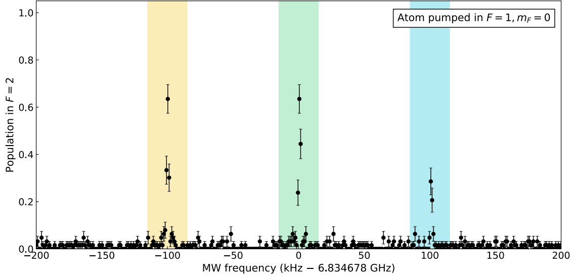
Figure 3.5: Resulting MW spectrum when the atom is initialized in F=1, m_F=0 . The colored yellow, green, and blue colored sections represent the transitions from F=1, m_F=0 to F=2, m_F=-1 , F=2, m_F=0 , and F=2, m_F=+1 respectively.
