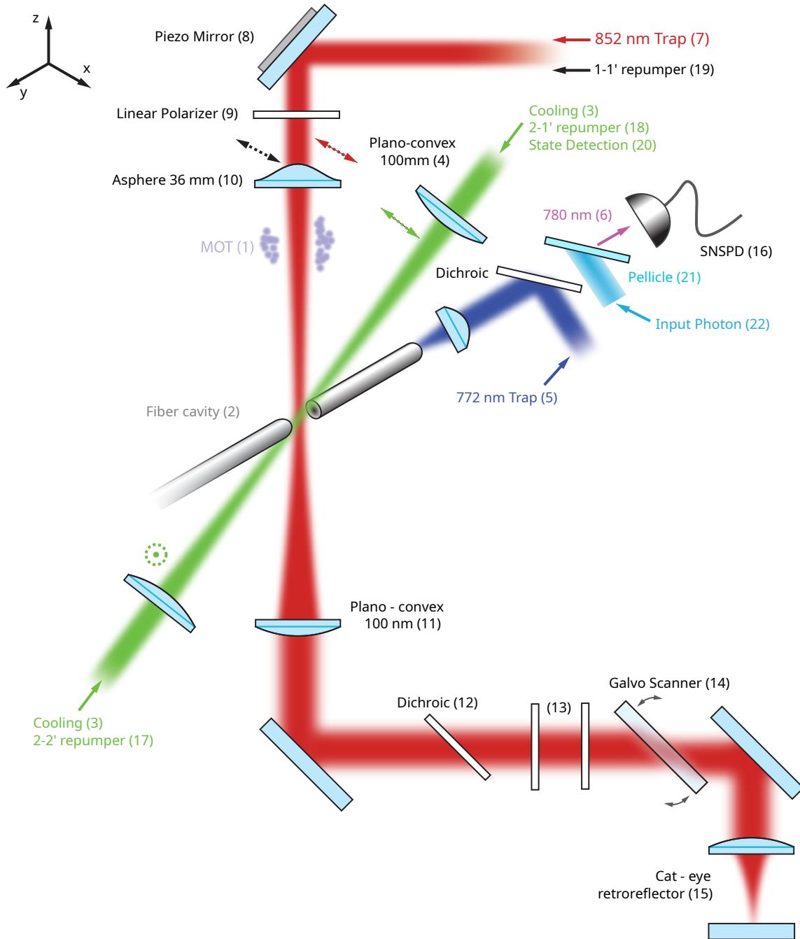
Figure 3.3: Overview of experimental setup used in this work. According to the reference frame, the z , the x , and the y axes are, respectively, the vertical trap, the long Cavity (not shown here), and the short Cavity axes. The dashed arrows and the dashed circle indicate the laser beams' polarization.
