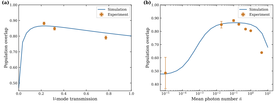
Figure 5.6: Comparison of the measured population overlap with the QuTiP master-equation simulation. (a) Population overlap as a function of the V-mode transmission, controlled by the number of intracavity Brewster windows. The three experimental points correspond to seven, five, and one Brewster windows (from left to right), with the mean input photon number fixed at \bar{n} \approx 0.1 . (b) Population overlap as a function of the mean input photon number \bar{n} , measured with seven Brewster windows installed. The overlap peaks near \bar{n} \approx 0.1 and decreases for both lower photon numbers, where vacuum contributions dominate, and higher photon numbers, where multi-photon components degrade the gate fidelity. Solid lines show the simulation results; markers indicate experimental data.
