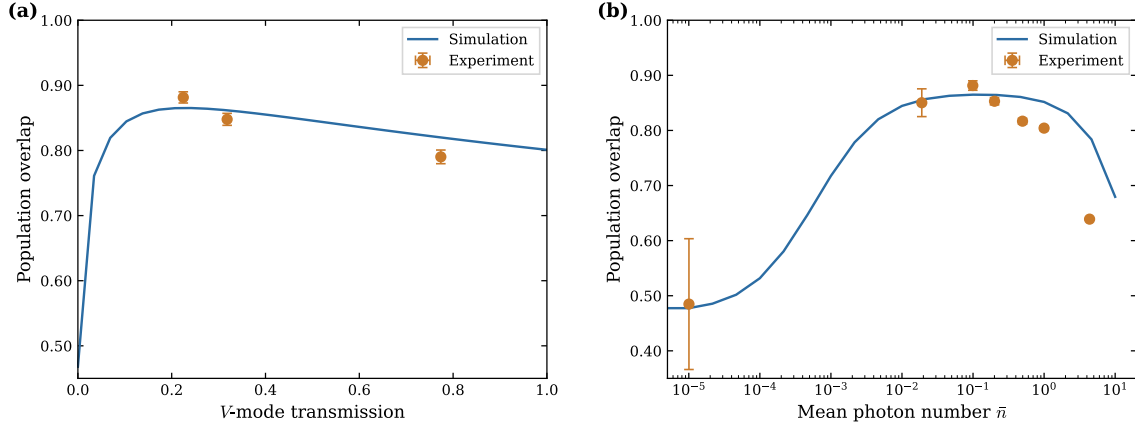
Figure 5.6: Comparison of the measured population overlap with the QuTiP master-equation simulation. (a) Population overlap as a function of the V-mode transmission, controlled by the number of intracavity Brewster windows. The three experimental points correspond to seven, five, and one Brewster windows (from left to right), with the mean input photon number fixed at \bar{n} \approx 0.1 . (b) Population overlap as a function of the mean input photon number \bar{n} , measured with seven Brewster windows installed. The overlap peaks near \bar{n} \approx 0.1 and decreases for both lower photon numbers, where vacuum contributions dominate, and higher photon numbers, where multi-photon components degrade the gate fidelity. Solid lines show the simulation results; markers indicate experimental data.
