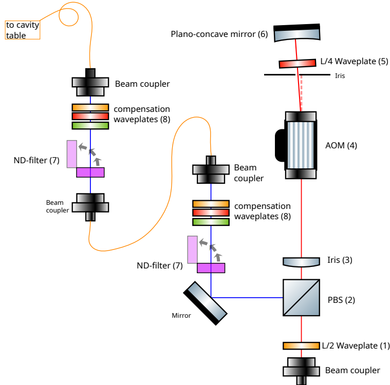
Figure 4.2: Double-pass AOM setup on the AOM table.
