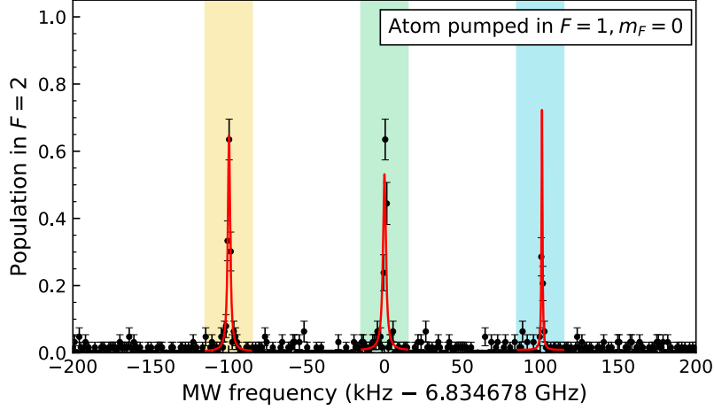
Figure 3.6: Resulting MW spectrum when the atom is initialized in F=1, m_F=0 . The yellow, green, and blue colored bands mark the transitions from F=1, m_F=0 to F=2, m_F=-1 , F=2, m_F=0 , and F=2, m_F=+1 , respectively. The red solid lines are Lorentzian fits to each of the three peaks, from which the transition frequencies and linewidths are extracted.
