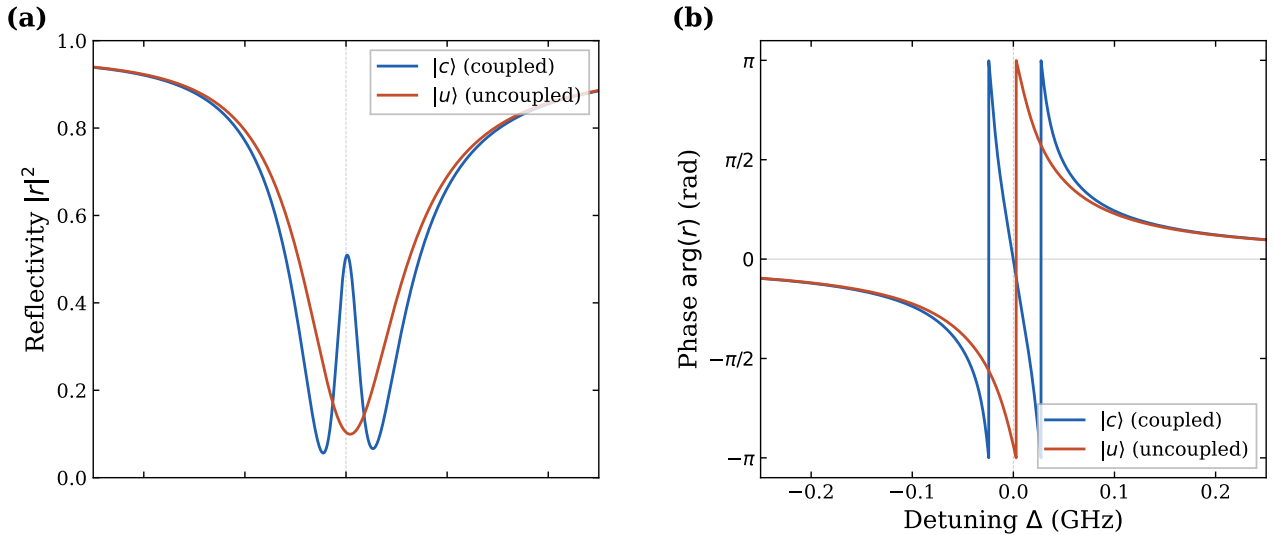
Figure 1: Simulated reflectivity (a) and phase (b) of the \pi -polarized cavity mode versus probe detuning, for the atom in the coupled state |c\rangle = |1\rangle (blue) and uncoupled state |u\rangle = |0\rangle (red). On resonance the reflected photon acquires a phase of 0 or \pi depending on the atomic state – the mechanism underlying the CPF gate.
