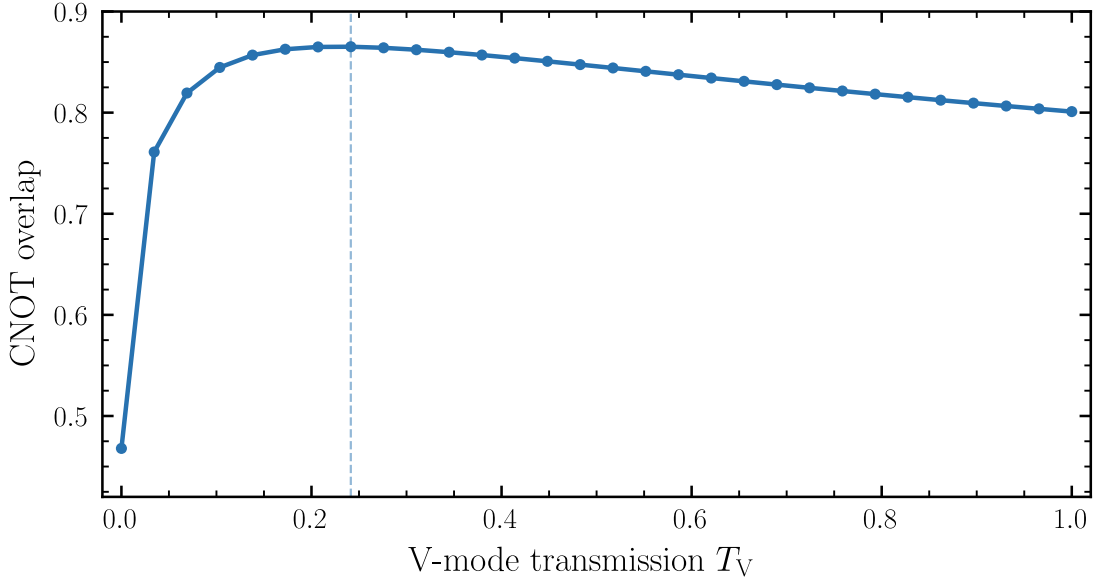
Figure A.1: Simulated CNOT gate overlap \mathcal{F} as a function of the V-mode cavity transmission T_V , obtained from a master-equation simulation of the atom–photon gate protocol. The dashed line marks the optimal transmission T_V^* \approx 0.24
