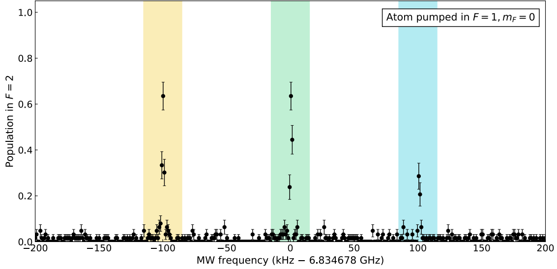
Figure 3.5: Resulting MW spectrum when the atom is initialized in F = 1, m_F = 0 . The colored yellow, green, and blue colored sections represent the transitions from F = 1, m_F = 0 to F = 2, m_F = -1 , F = 2, m_F = 0 , and F = 2, m_F = +1 respectively.
