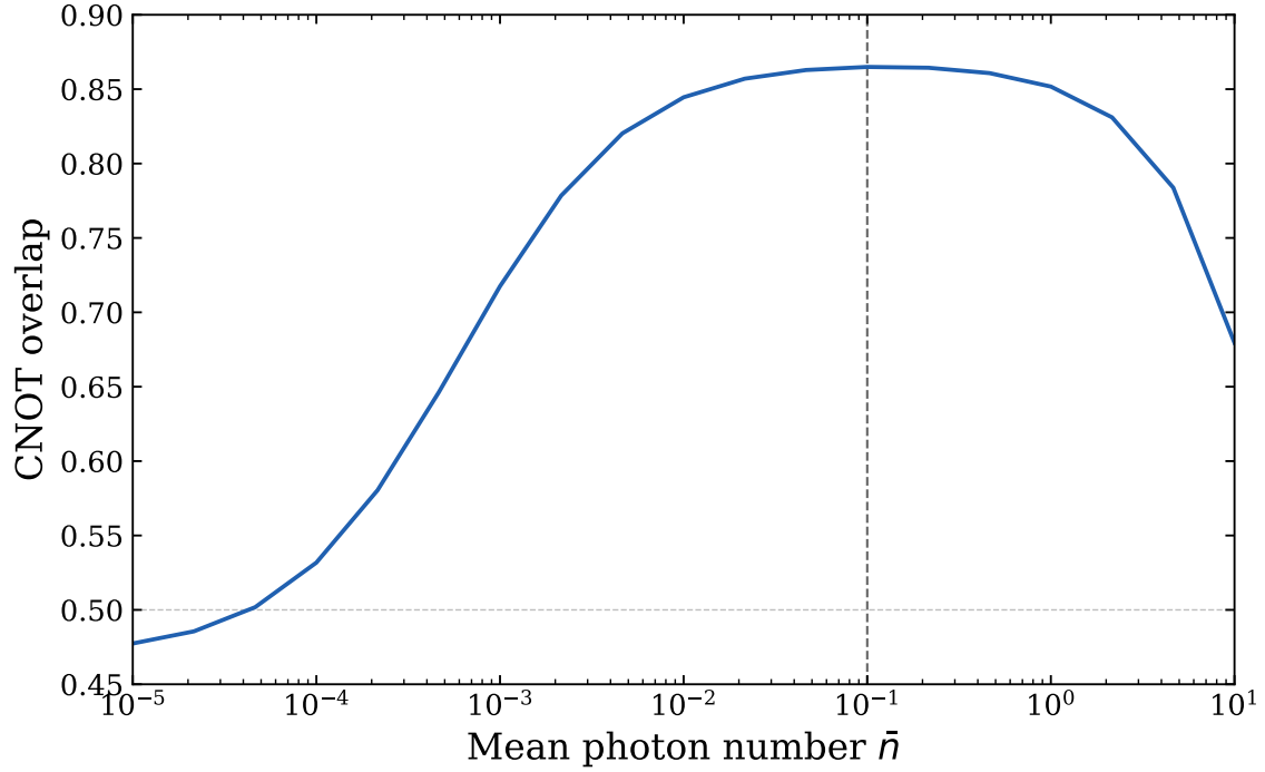
Figure A.2: Simulated CNOT gate overlap as a function of the mean input photon number \bar{n} . The V-mode transmission is fixed at T_V = 0.2247 and the Fock space is truncated at N_{\text{ph}} = 3 . The dashed line marks the optimal mean photon number \bar{n}^* \approx 0.10 , at which the overlap reaches a maximum of \approx 0.865 .
