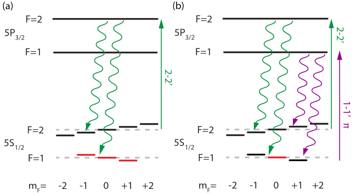
Figure 3.4: Schemes utilized for OP in F = 1 (a), and F = 1, m_F = 0 (b). Each sketch shows the used lasers (straight arrows), the atomic decay (wavy arrows), and the targeted state (red lines). [38]
