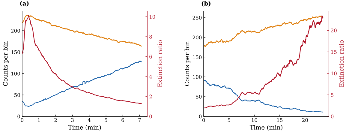
Figure 5.7: Long-term drift of the polarization extinction ratio measured on the gate photon reflection path, recorded at the two SNSPD channels of the polarization analysis stage (Ch 4 and Ch 7) when sending L polarized light. In each panel, the Ch 4 (blue) and Ch 7 (orange) count rates per 25 ms bin are shown on the left y-axis, while the corresponding extinction ratio \eta = N_{\text{Ch 7}}/N_{\text{Ch 4}} is shown on the right y-axis (red). (a) Drift recorded with the UV LED switched on: the extinction ratio rises sharply within the first minute and then decays monotonically as Ch 4 counts gradually increase and Ch 7 counts decrease, indicating a continuous rotation of the analysed polarization. (b) Drift recorded after a 5 minute measurement where the atom was prepared in |0\rangle and L polarized light was sent: Ch 4 counts decrease and Ch 7 counts increase over the full 24 min measurement window, driving the extinction ratio from \eta \approx 2 up to \eta \approx 23 .
