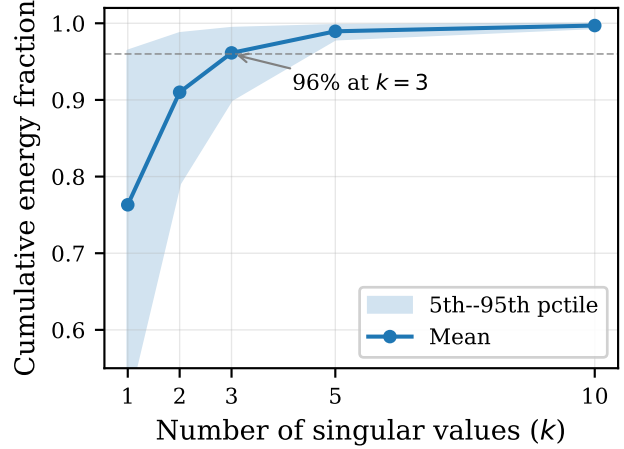
Figure 1. Cumulative energy fraction vs. number of singular values, averaged over 500 matchups (5th–95th percentile envelope). The top 3 singular values capture 96% of spectral energy, revealing that VGC turn-1 is a 3-dimensional game in a \sim 122 -dimensional action space.
