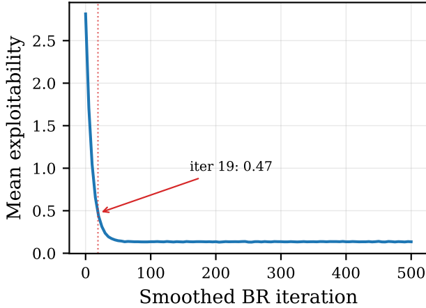
Figure 3. Smoothed best-response convergence from BC initialization. Exploitability decreases from 2.81 to below 0.50 in \sim 19 iterations, reaching 0.14 at iteration 500.
