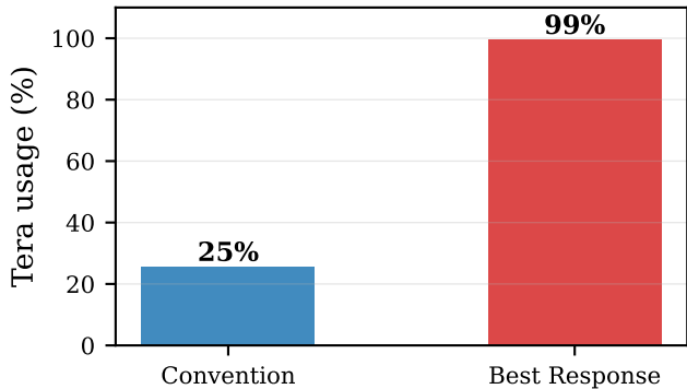
(a) Terastallization
