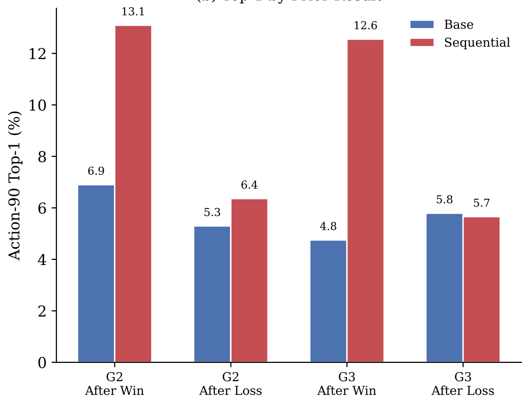
(b) Top-1 by Prior Result
