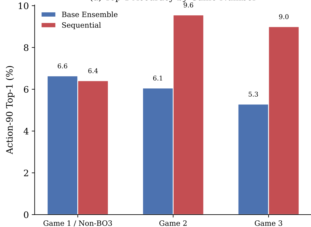
(a) Top-1 Accuracy by Game Number
