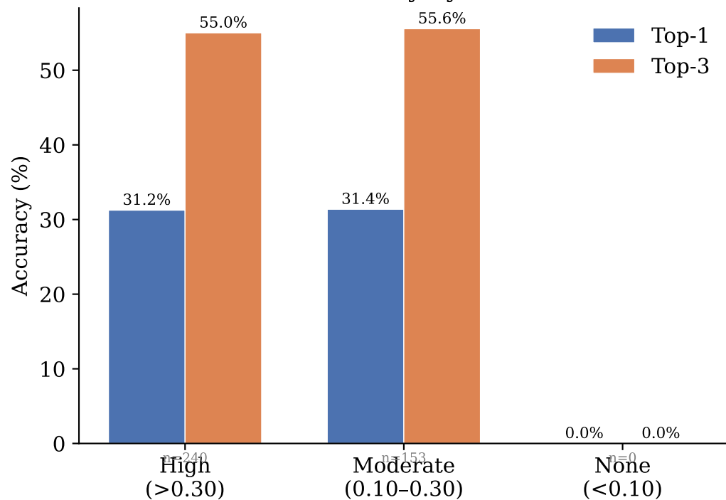
Lead-2: Accuracy by Consensus
