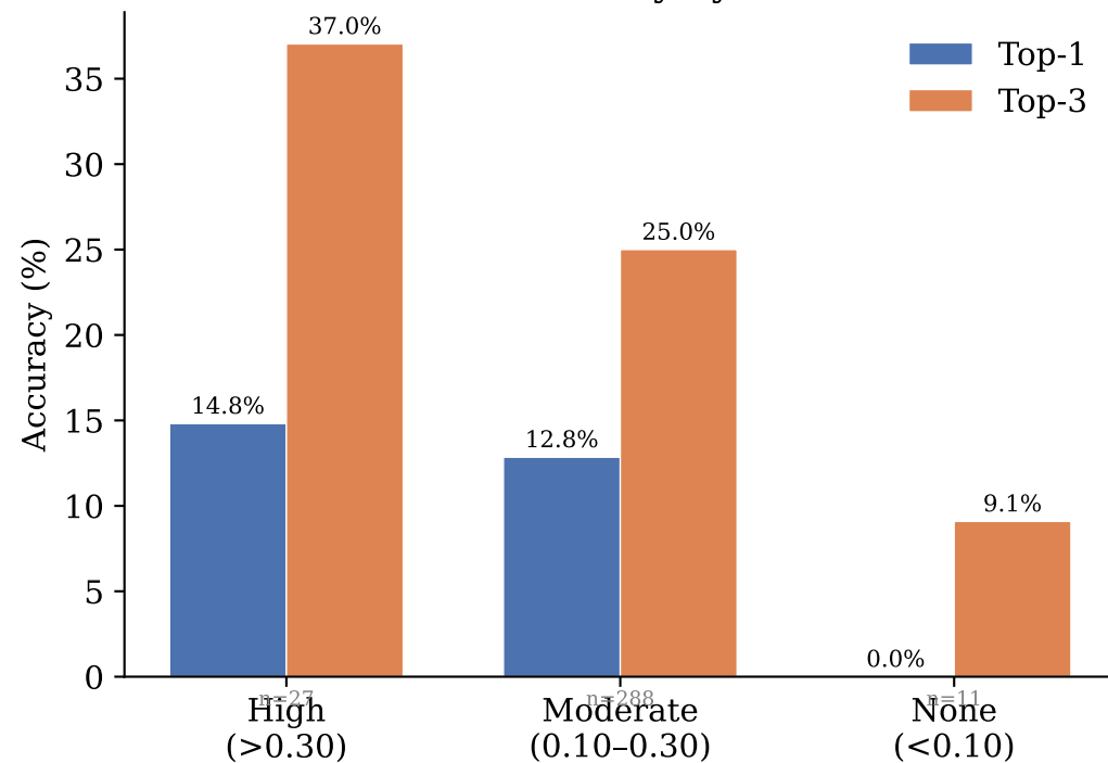
Action-90: Accuracy by Consensus
