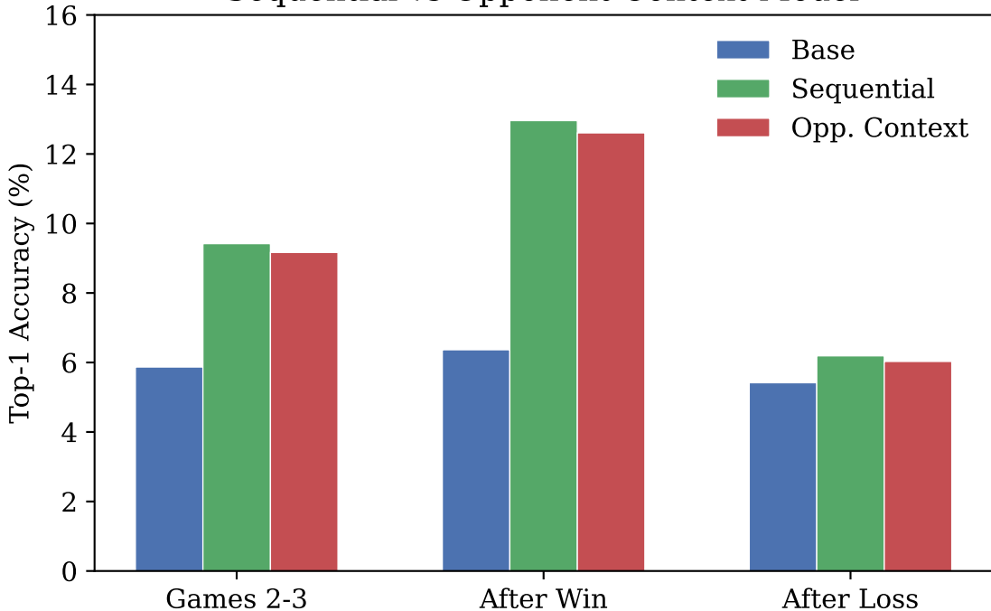
Sequential vs Opponent-Context Model
