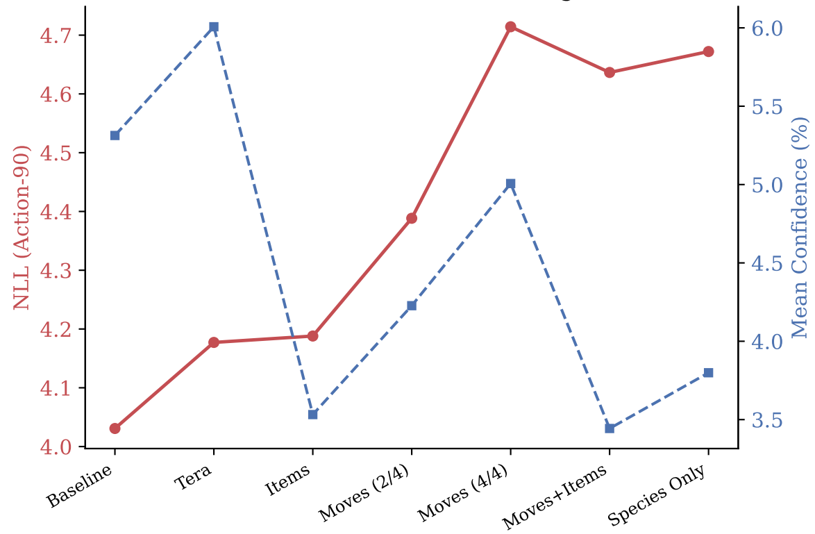
NLL and Confidence vs Masking Level
