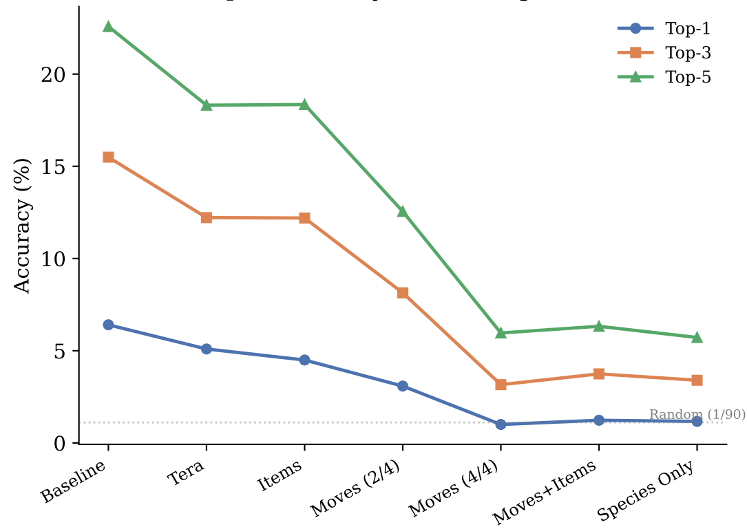
Top-k Accuracy vs Masking Level
