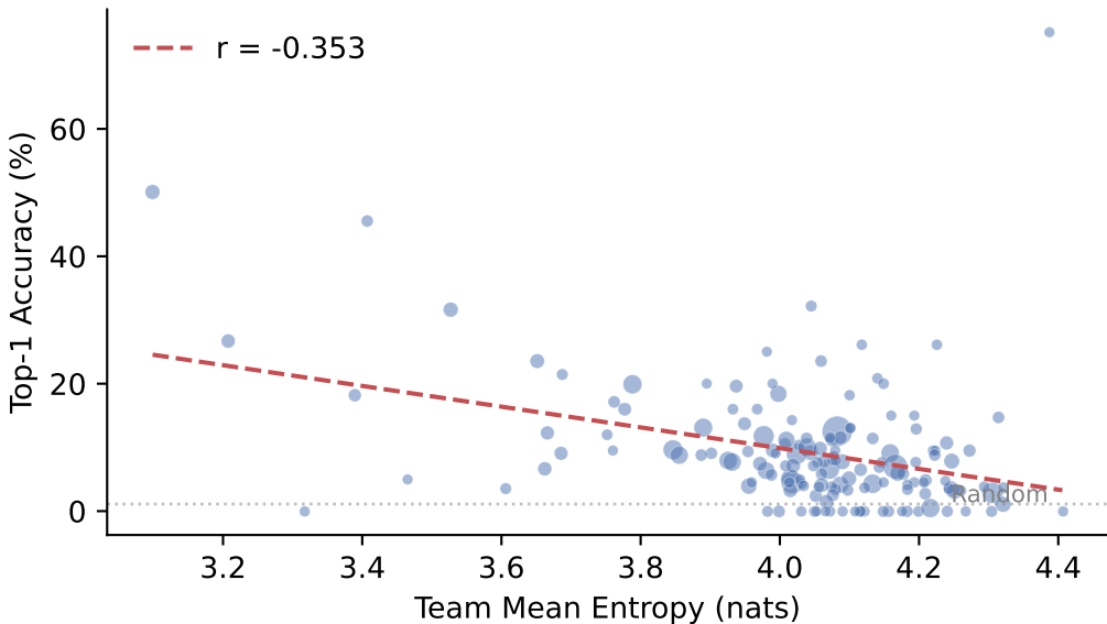
Entropy vs Top-1 Accuracy
