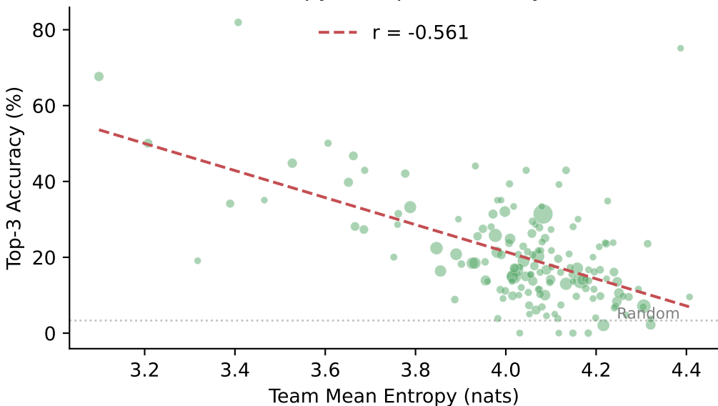
Entropy vs Top-3 Accuracy
