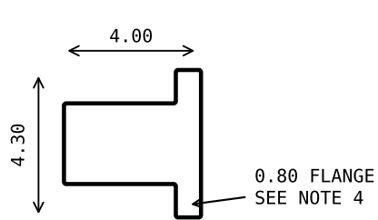
VIEW A - END
