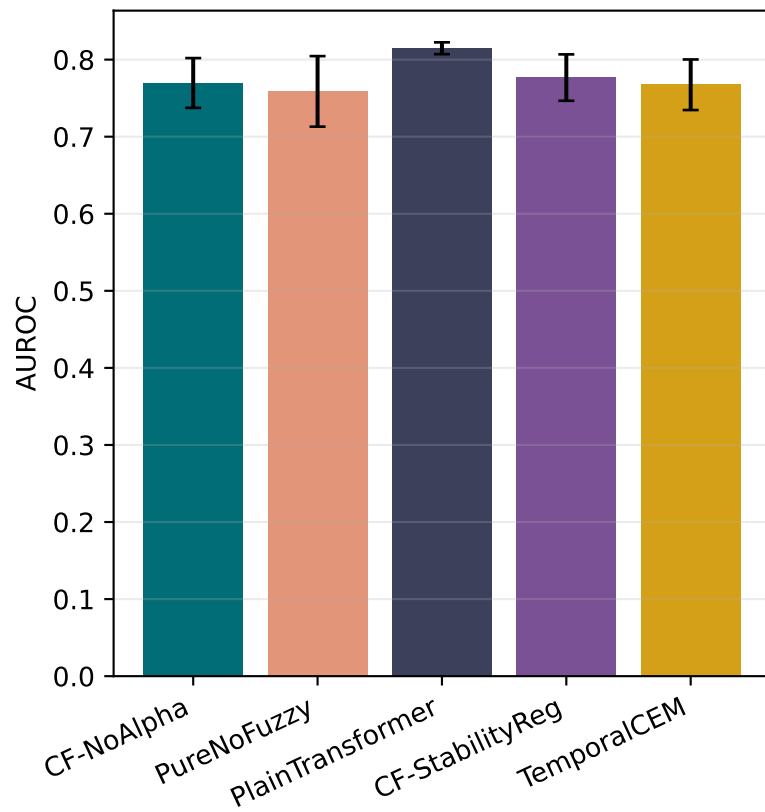
Held-out predictive performance and calibration across 30 runs
