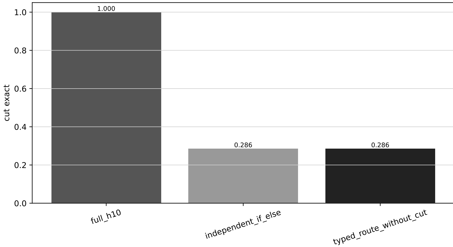
Minimal-cut exact match on composite routes (development only)
