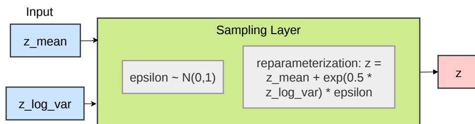
Gambar 3.6. Diagram aliran Reparameterization Layer
