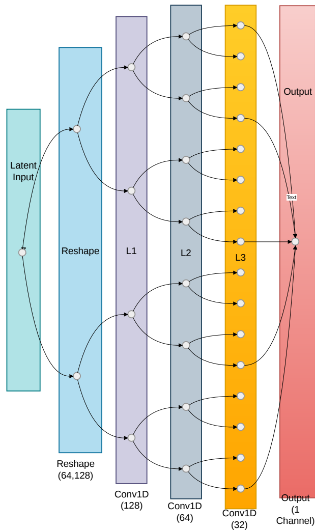
Gambar 3.7. Diagram aliran Decoder Layer
