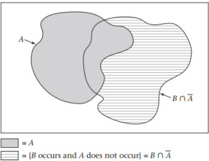
Diagrammatic representation of the addition law of probability for independent events
