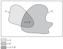
Diagrammatic representation of the addition law of probability
