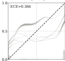
P(I Know)
