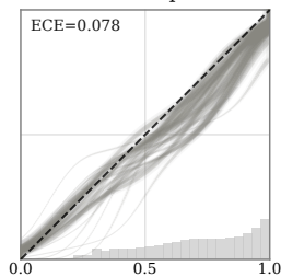
InternalInspector
