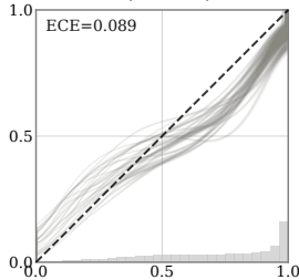
P(I Know)
