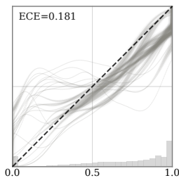
CCPS
