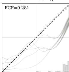
Self-Probing
