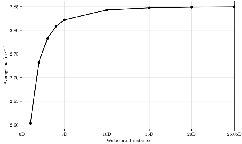
Figure 25: The weighted average of the velocity in the rotorplane calculated at different cutoff distances.
