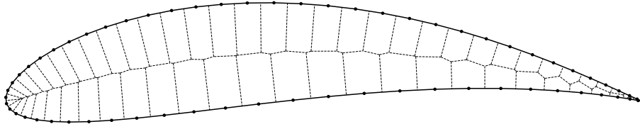
Figure 27: VORONOI diagram of the VON KÁRMÁN–TREFFTZ airfoil (dashed).
