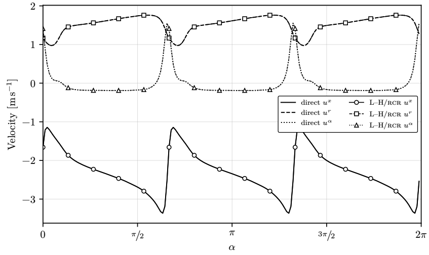
Figure 16: The induced velocity at the rotorplane, for r/R = 0.8 .
