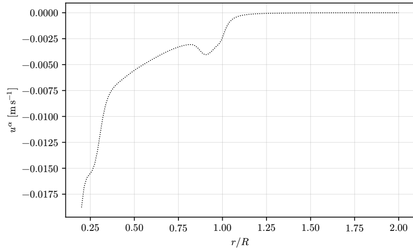
Figure 23: The average over the azimuth of the azimuthal velocity component.
