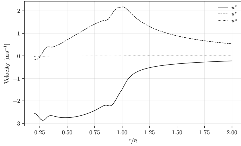
Figure 22: The average over the azimuth of all three cylindrical velocity components.
