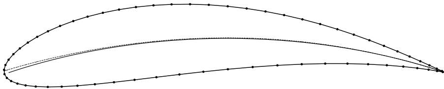
Figure 29: Mean camber line (dashed) and skeleton (full) of the VON KÁRMÁN–TREFFTZ airfoil.
