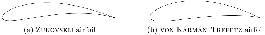
Figure 4: Two airfoils described respectively by equations (3.2) and (3.9), whose parameters are c = 1.4 and s = 1/4(i - 3/5) . The trailing edge parameter is k = 1.94 .
