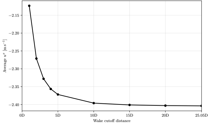
Figure 24: The velocity component u^x in the rotorplane calculated at different cutoff distances.
