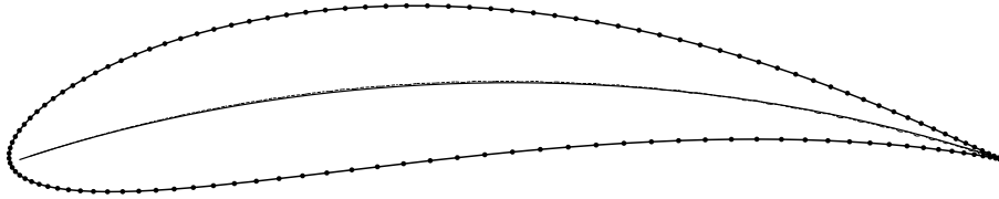
Figure 28: Medial axis of the VON KÁRMÁN–TREFFTZ airfoil (dashed), and the skeleton (full).
