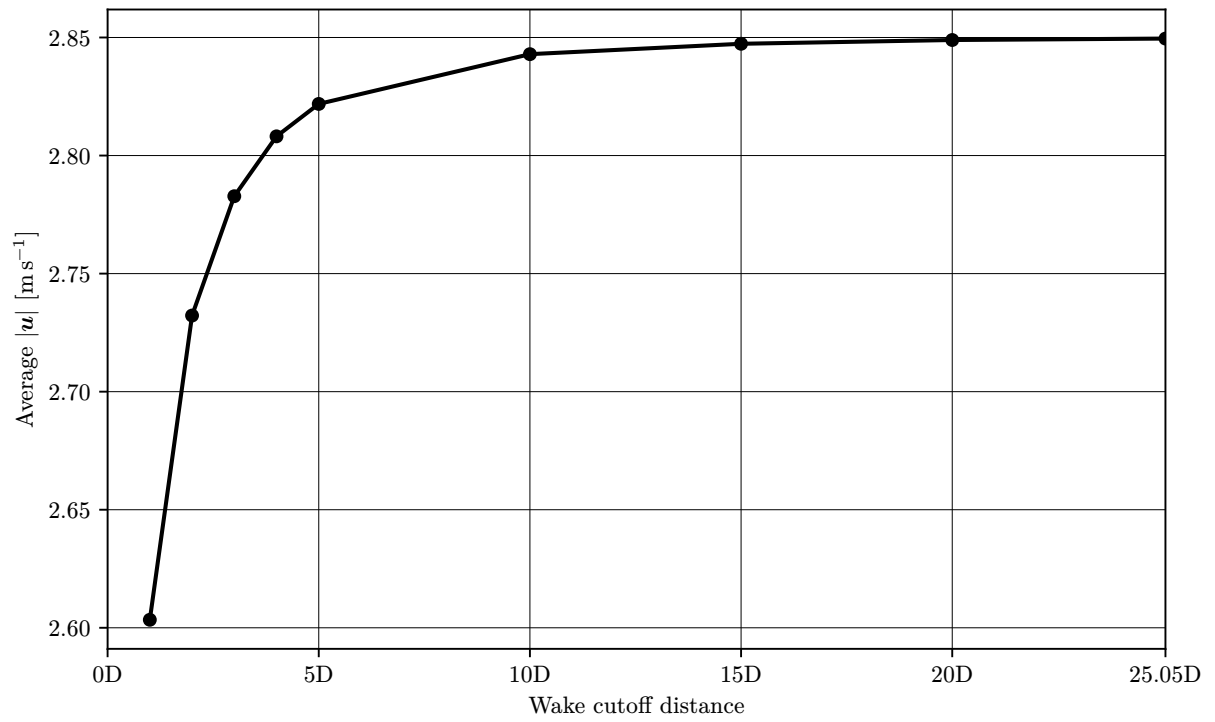
Figure 14: The weighted average of the velocity in the rotorplane calculated at different cutoff distances.
