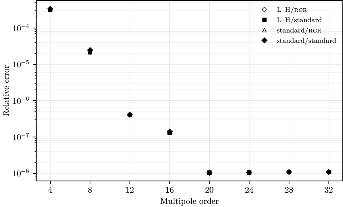
Figure 10: The relative error of the multipole induced velocity to the direct calculation in the rotorplane.
