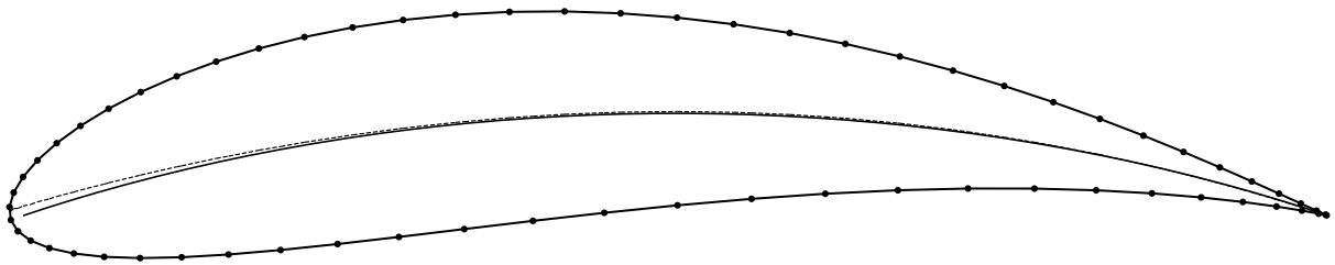
Figure 16: Mean camber line with skeleton of the VON KÁRMÁN–TREFFTZ airfoil
