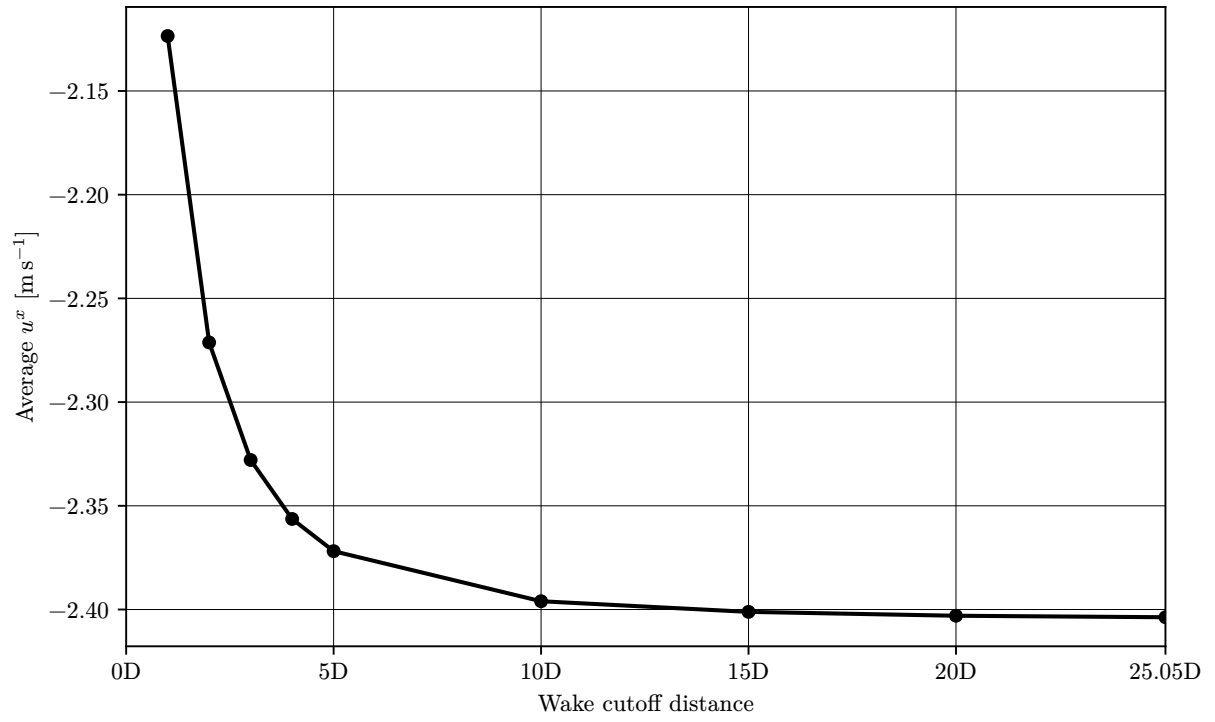
Figure 13: The velocity in the rotorplane along x calculated at different cutoff distances.
