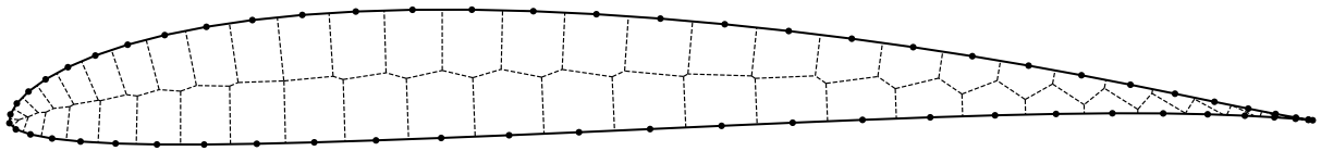
Figure 18: VORONOI diagram of SD7032
