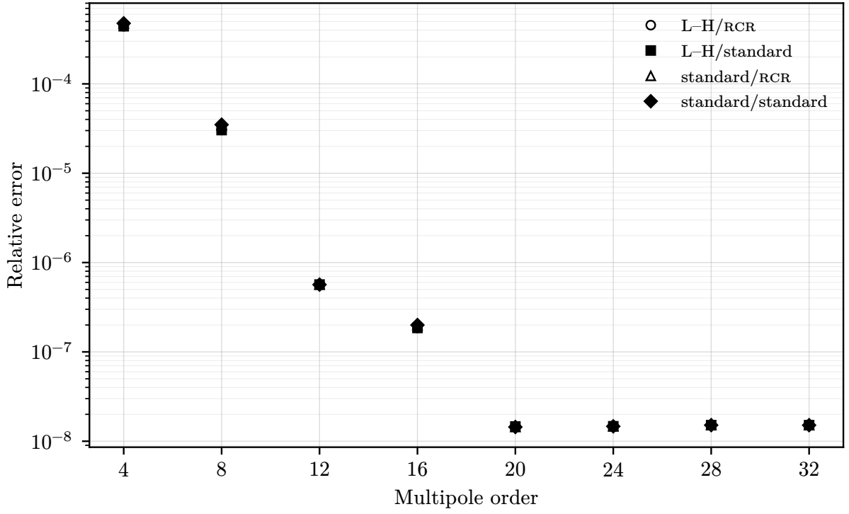
Figure 11: The relative error of the multipole induced velocity to the direct calculation at x = -0.1D .
